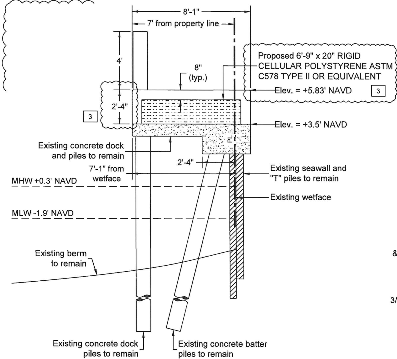
Dock Section "A" Scale 1/4" = 1'-0"
