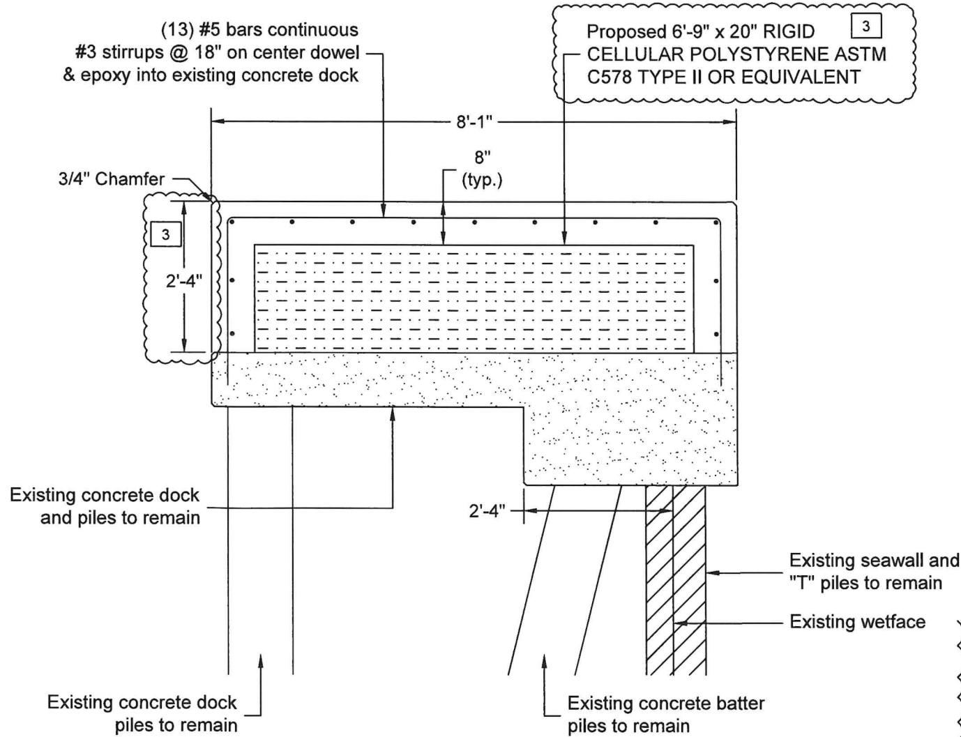
Dock Steel Detail "A" Scale: 1/2" = 1'-0"
