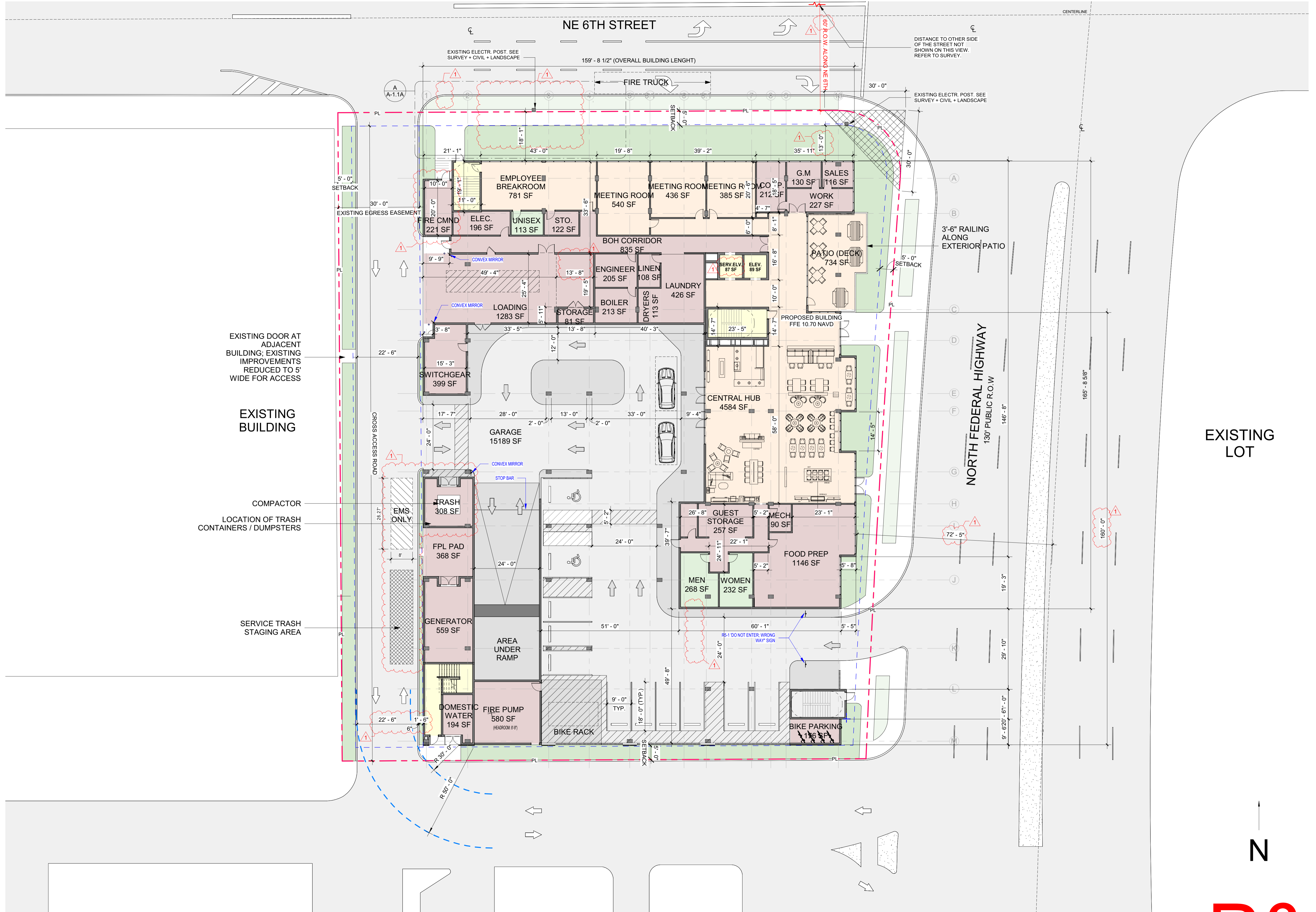
① LEVEL 1 - FLOOR PLAN 1/16" = 1'-0"
