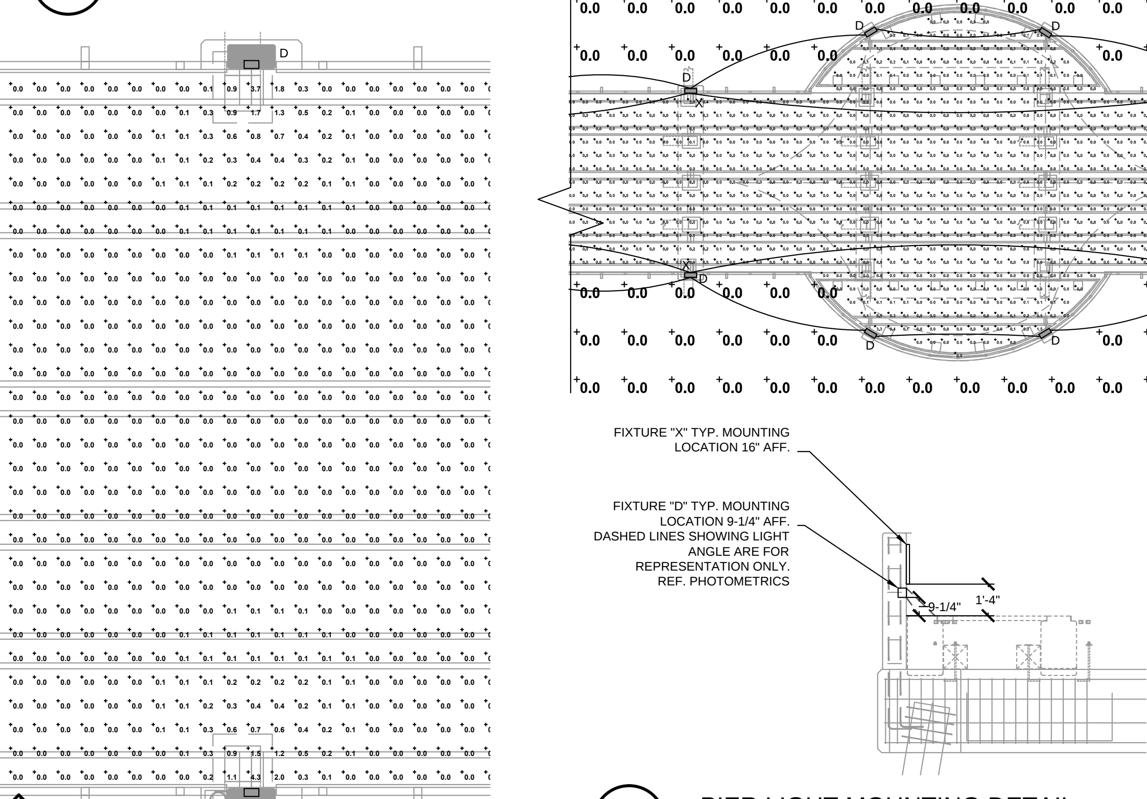
3 ENLARGED PIER LIGHTING SCALE: 1/4" = 1'-0"
