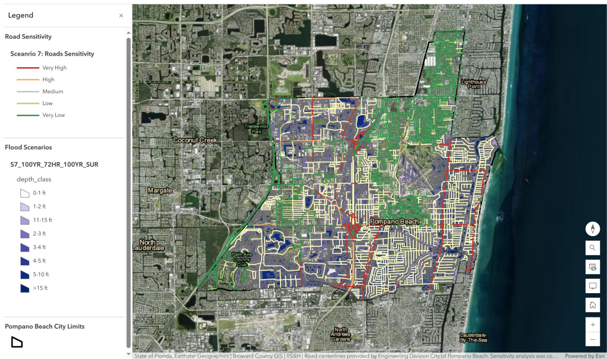
Figure 9: City Roadway Sensitivity under Scenario 7 (RS&H)
