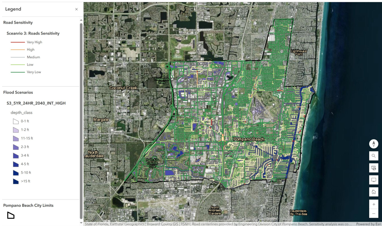
Figure 7: City Roadway Sensitivity under Scenario 3 (RS&H)
