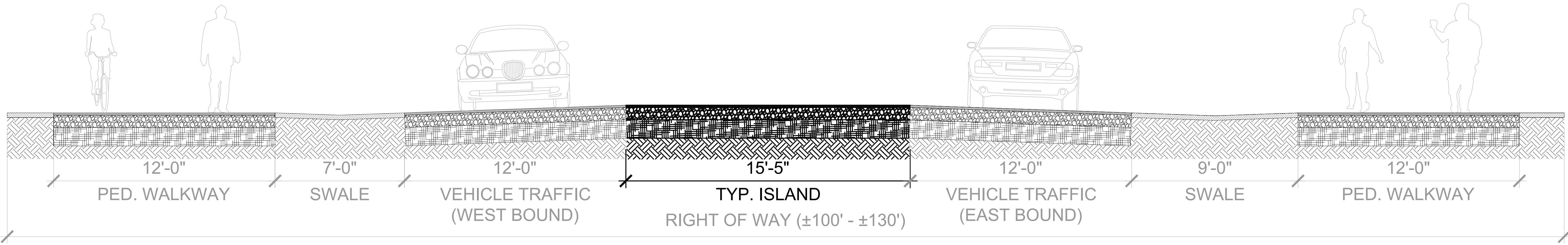
EXISTING TYPICAL ISLAND SECTION
