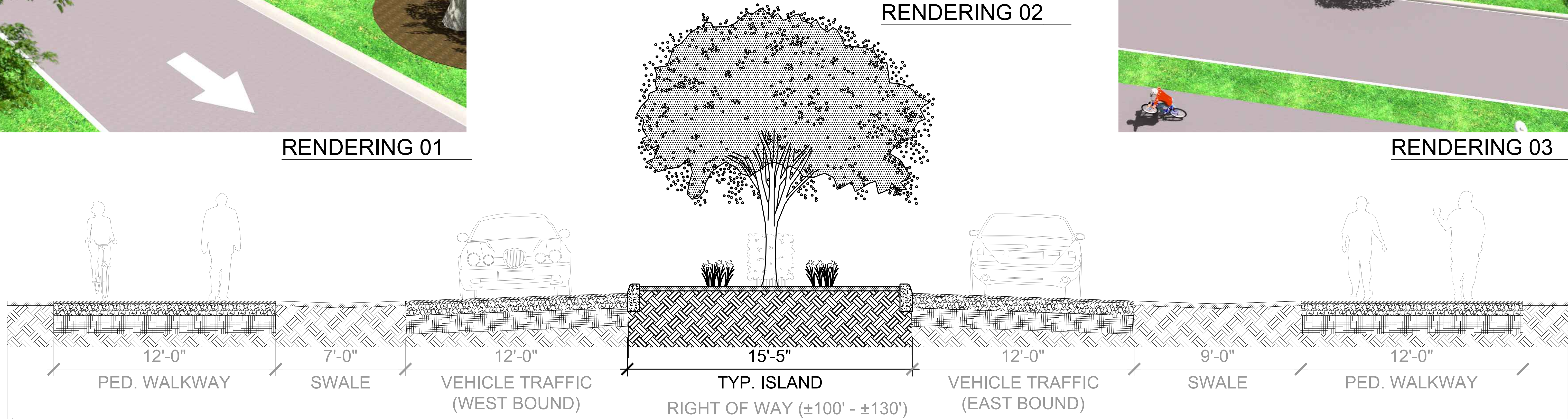
PROPOSED TYPICAL ISLAND SECTION (1-8)
