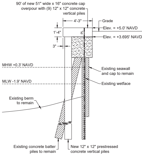
Seawall Section Scale 1/4" = 1'-0"
