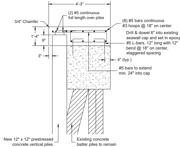
Cap Steel Detail Scale: 1/2" = 1'-0"
