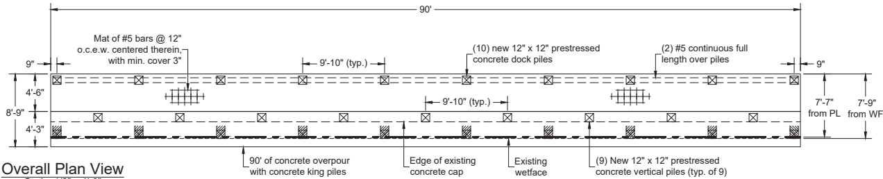
Overall Plan View Scale: 1/8" = 1'-0"
