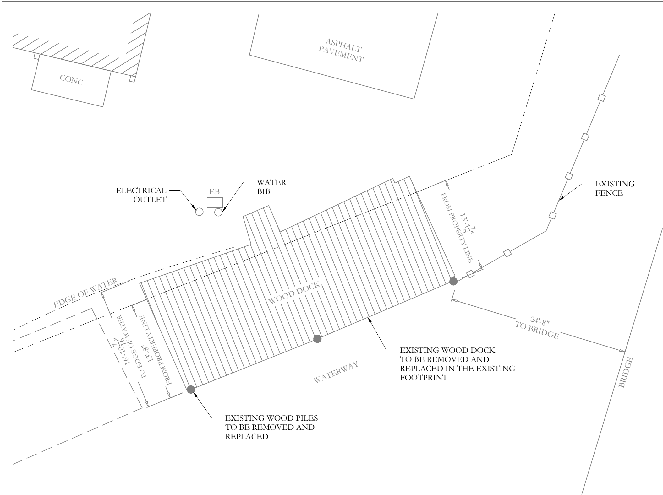
EXISTING CONDITIONS LAYOUT SCALE: 1/8" = 1'-0"
