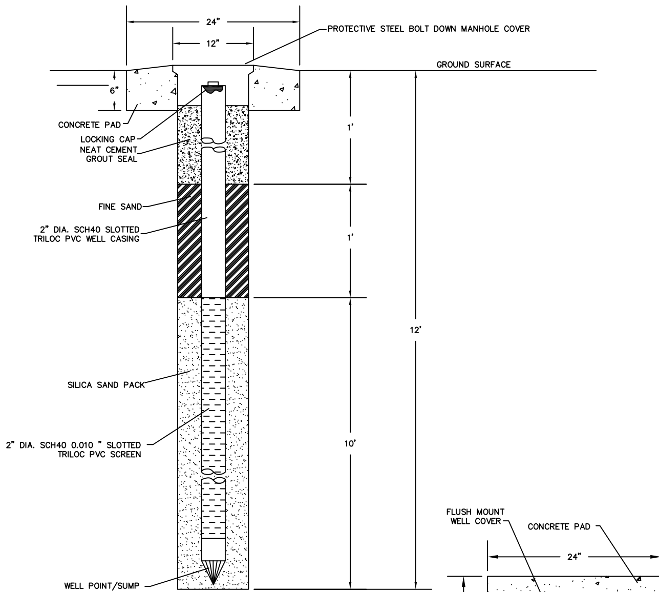
SECTION VIEW
