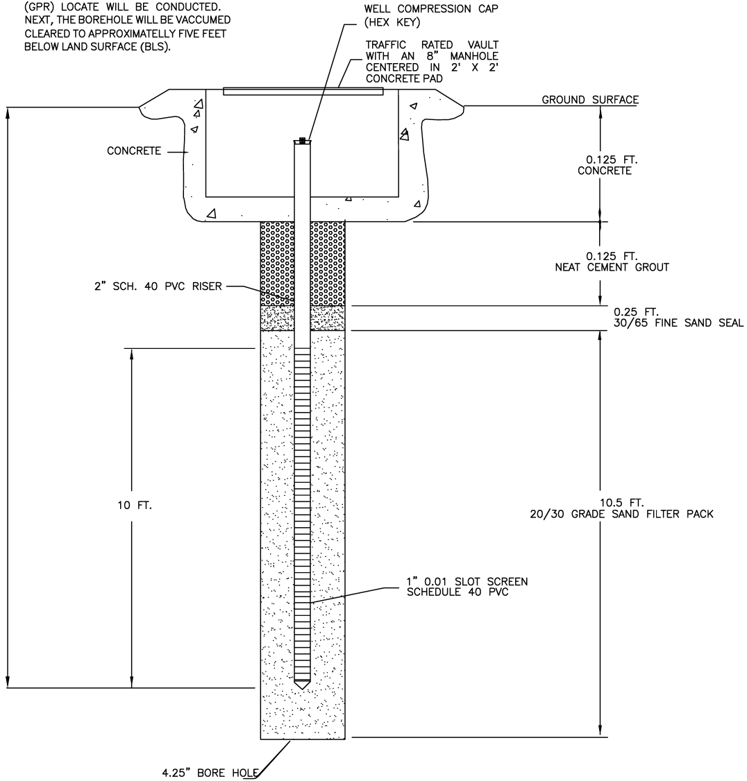
PROPOSED MONITORING WELL(S) CONSTRUCTION DETAILS NOT TO SCALE
