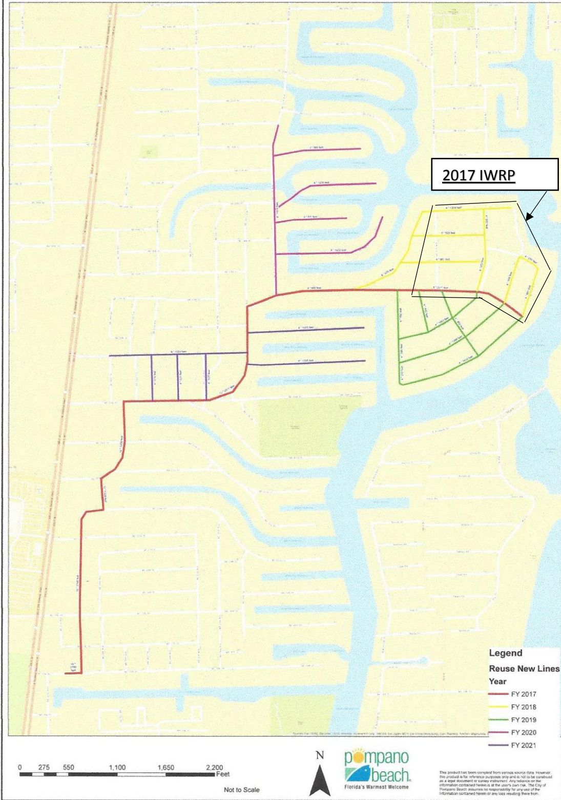
Figure 1. City of Pompano Beach Proposed Reuse Lines
