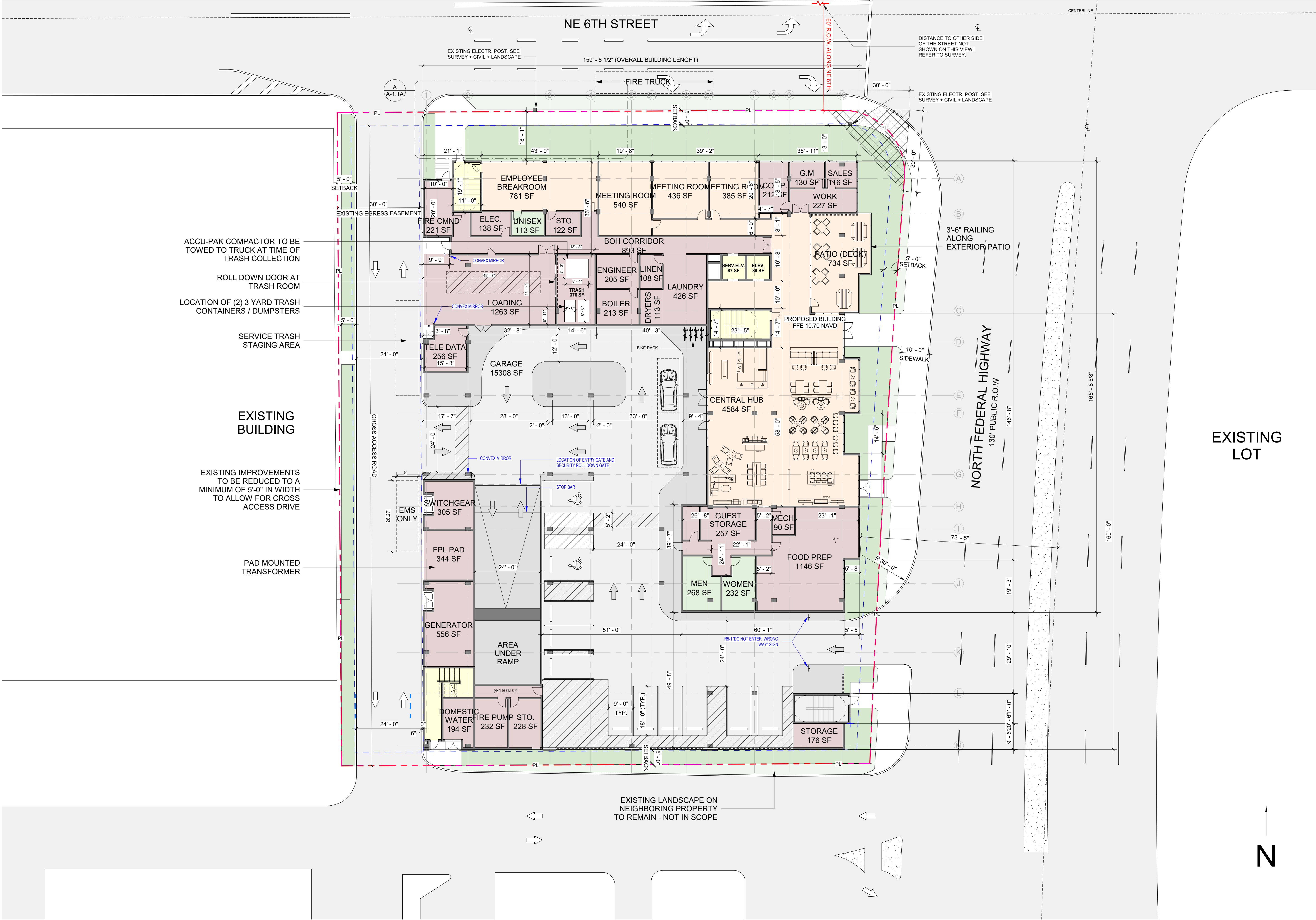
1 LEVEL 1 - FLOOR PLAN 1/16" = 1'-0"
