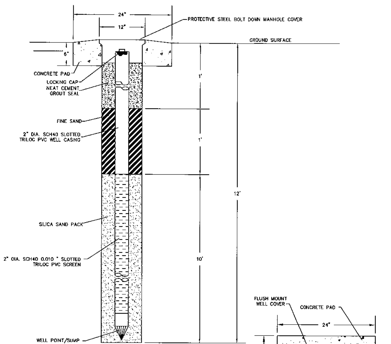
SECTION VIEW
