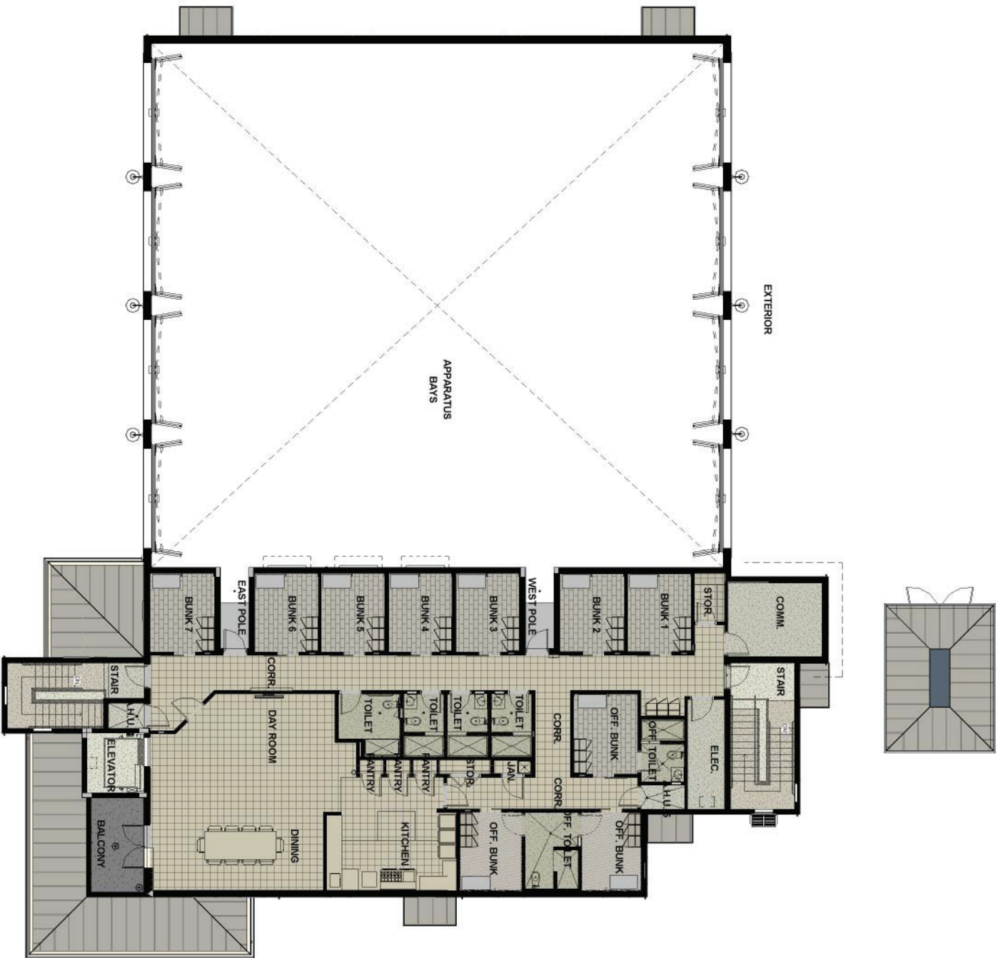
1 SECOND FLOOR PLAN 1/8" = 1'-0" 4,049 S.F.
